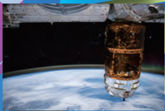
©JAXA/NASA
